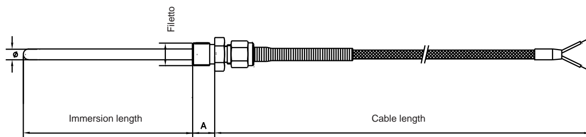
TR1 B: with adjustable compression fitting
