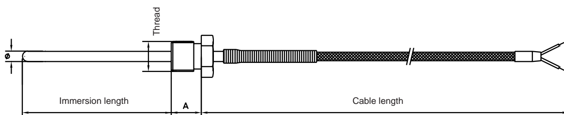
TR1 C: with welded fitting
