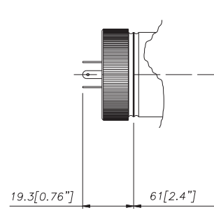
M - 4-pole connector microsolenoid
