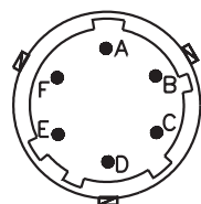
Male Connector VPT02A10-6PT2
