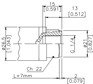
(4) G 1/4 FEMALE
