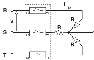
Three-phase Star control with neutral
