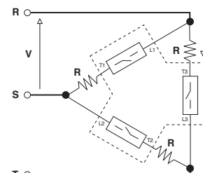
Three-phase Triangle open control
