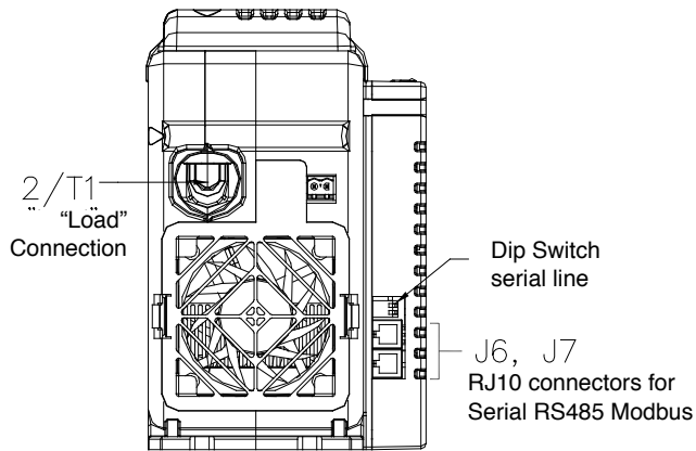
Low view WITH option RS485 serial line
