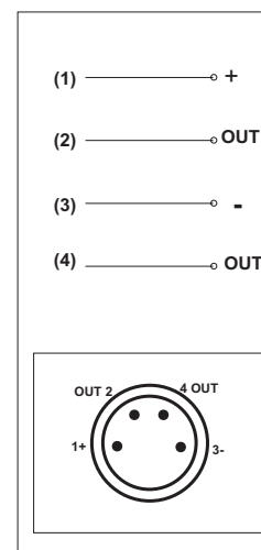
V8M 4 POLI/ 4 WIRES
