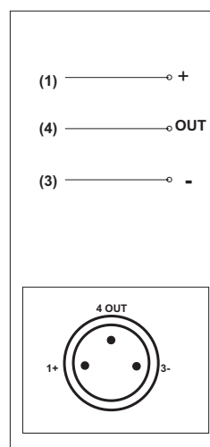
V6M 3 POLI/ 3 WIRES
