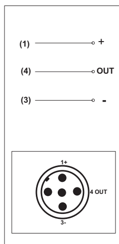
CA - CB 3 POLI/ 3 WIRES
